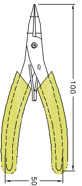
Micro bent nose pliers
